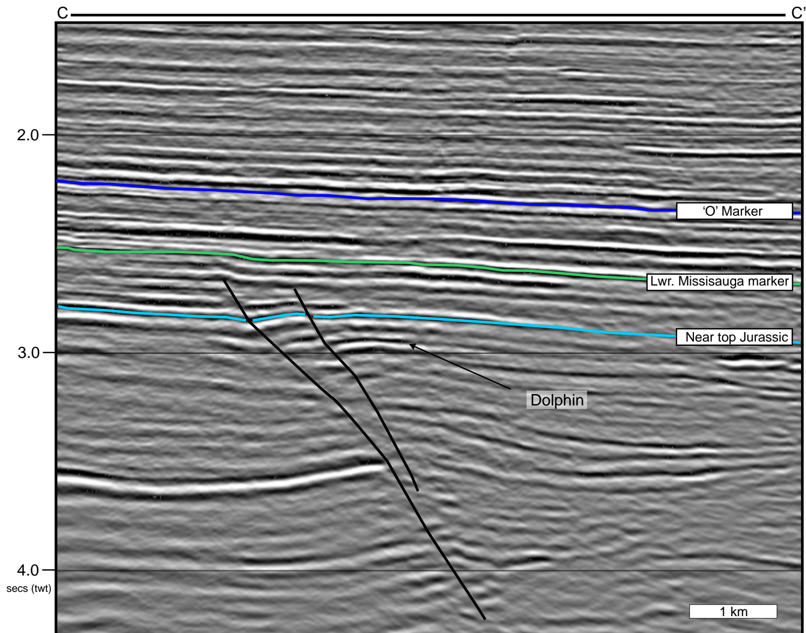
Seismic profile C-C' through the Dolphin prospect.
