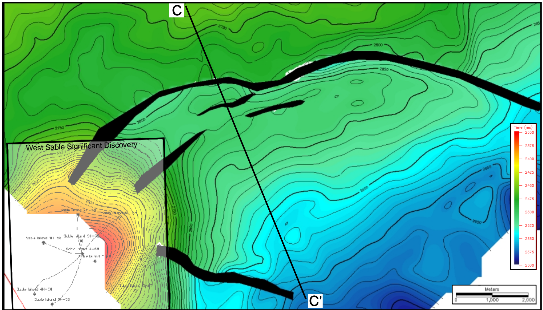
Structure map of a near top Jurassic seismic marker showing the Dolphin prospect and the location of seismic profile C-C'. The West Sable Significant Discovery area is highlighted in the lower left of the figure.
