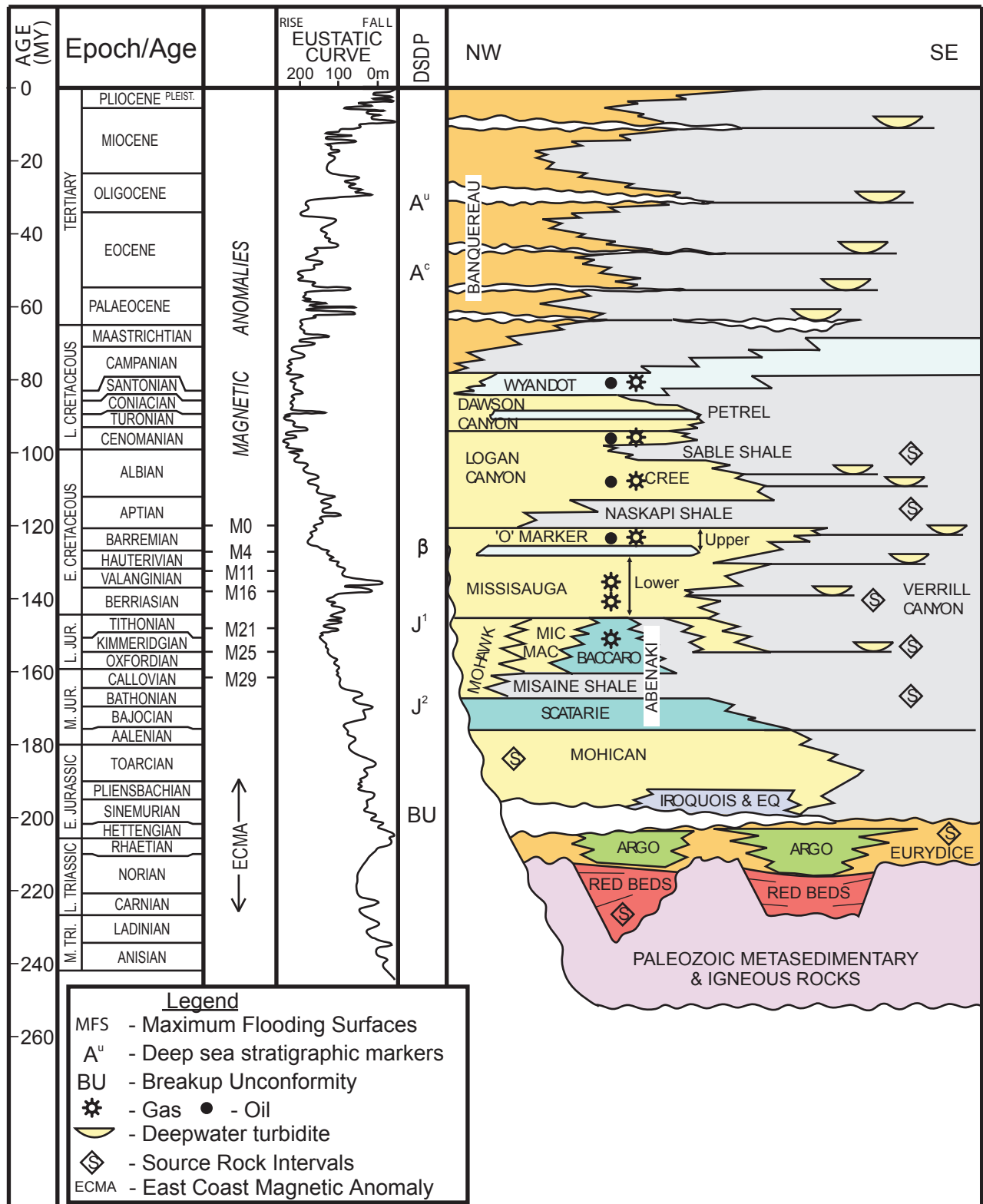
Figure 4: Generalized stratigraphic column for the Scotian Basin, offshore Nova Scotia (CNSOPB). Detailed columns can be found in Wade & MacLean (1990). Sea level curve from Haq et al. (1987). Time scale from Gradstein & Ogg (2004). Stratigraphy modified from Wade et al (1993, 1995).
