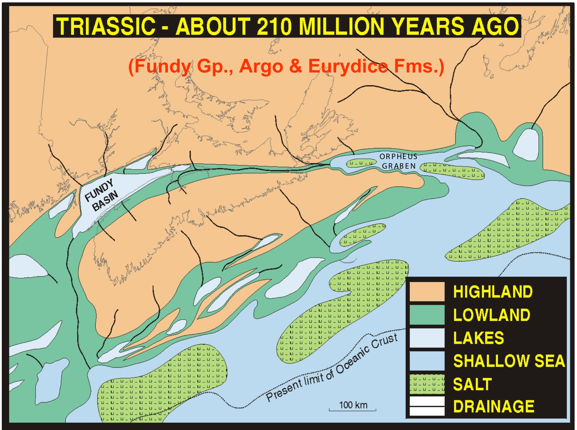
Figure 5: Simplified paleogeographic reconstruction of the Scotian Basin during the Late Triassic (Rhaetian) ca. 210 mya. Salt deposition likely was initiated during this period although on a much smaller scale than illustrated here. Argo formation salts of this age have yet to be sampled in this basin but are present on the southeast Grand Banks. Copyright © Atlantic Geoscience Society – used with permission.
