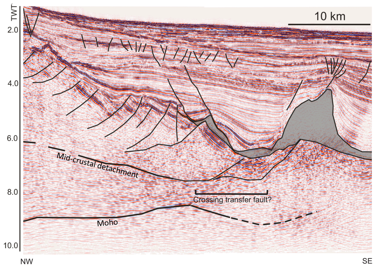
Figure 10 – Close-up seismic profile of middle parts of Figure 2 (SD to proximal ASM province), showing prominent northwest-dipping faults that may detach in a mid-crustal detachment surface. Slow water column velocities were depth converted, but remaining section is in TWT.
