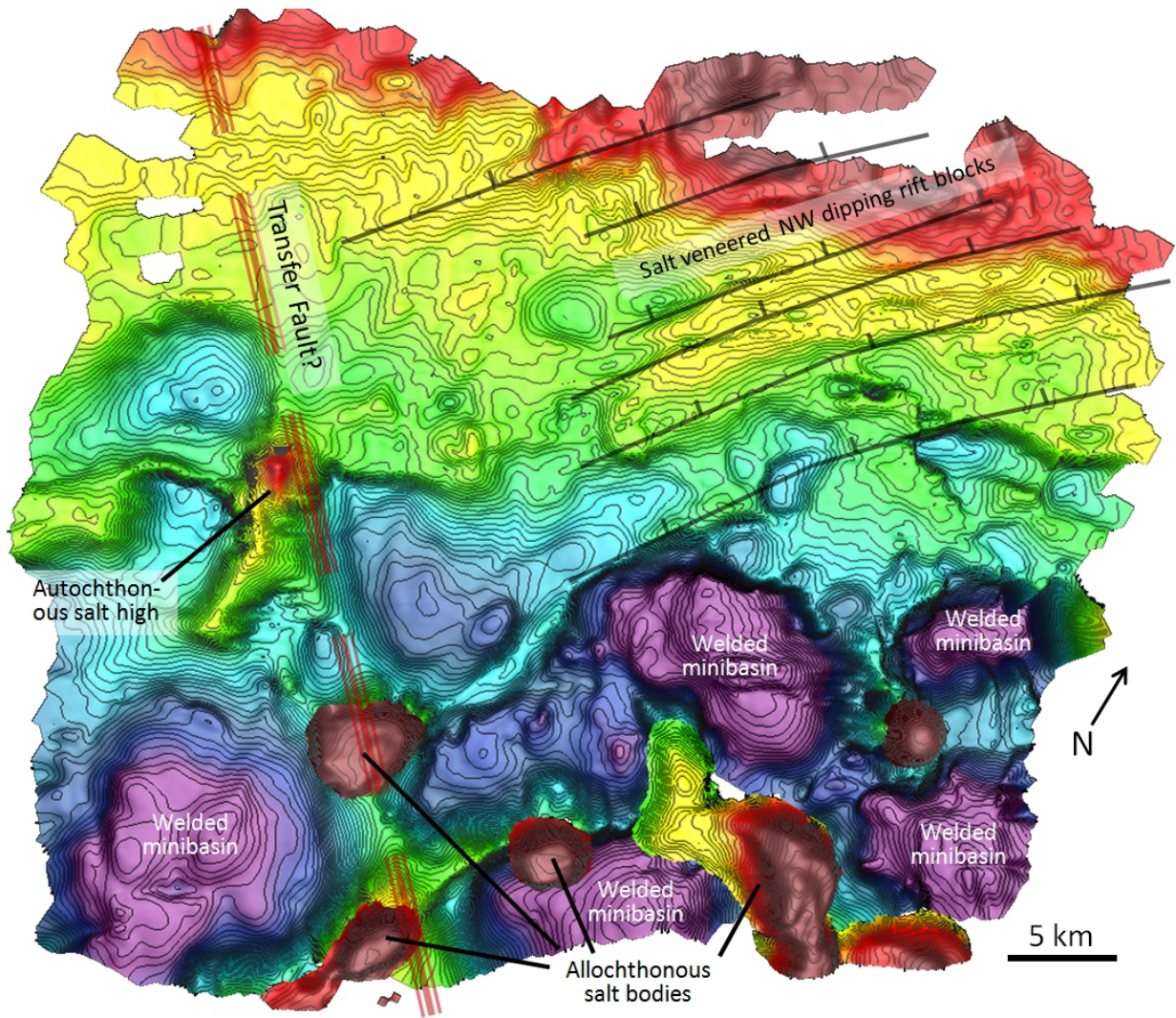
Figure 11 – Close-up of the top autochthonous salt to primary weld marker, showing the synrift 'fabric' produced by underlying rift blocks, with offsets on minibasins interpreted to be caused by a transfer fault. The figure also illustrates the transition from the SD province to the ASM province where allochthonous salt bodies were expelled from a chain of minibasins along the base of the image. Shallow areas are red, deep areas are purple. See Figure 1a for location.
