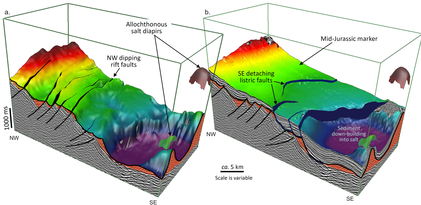
Figure 12 – a) Perspective view sculpted along the top autochthonous salt to primary weld marker, showing the synrift fabric below a thin veneer of autochthonous salt. The landward-dipping (northwest) extensional basement faults are well imaged; b) Perspective view showing a series of seaward dipping listric faults within Jurassic cover strata that sole out into the thin autochthonous salt layer. Fault vergence is in the opposite direction of the northwest-dipping synrift faults. See Figure 1a for location.
