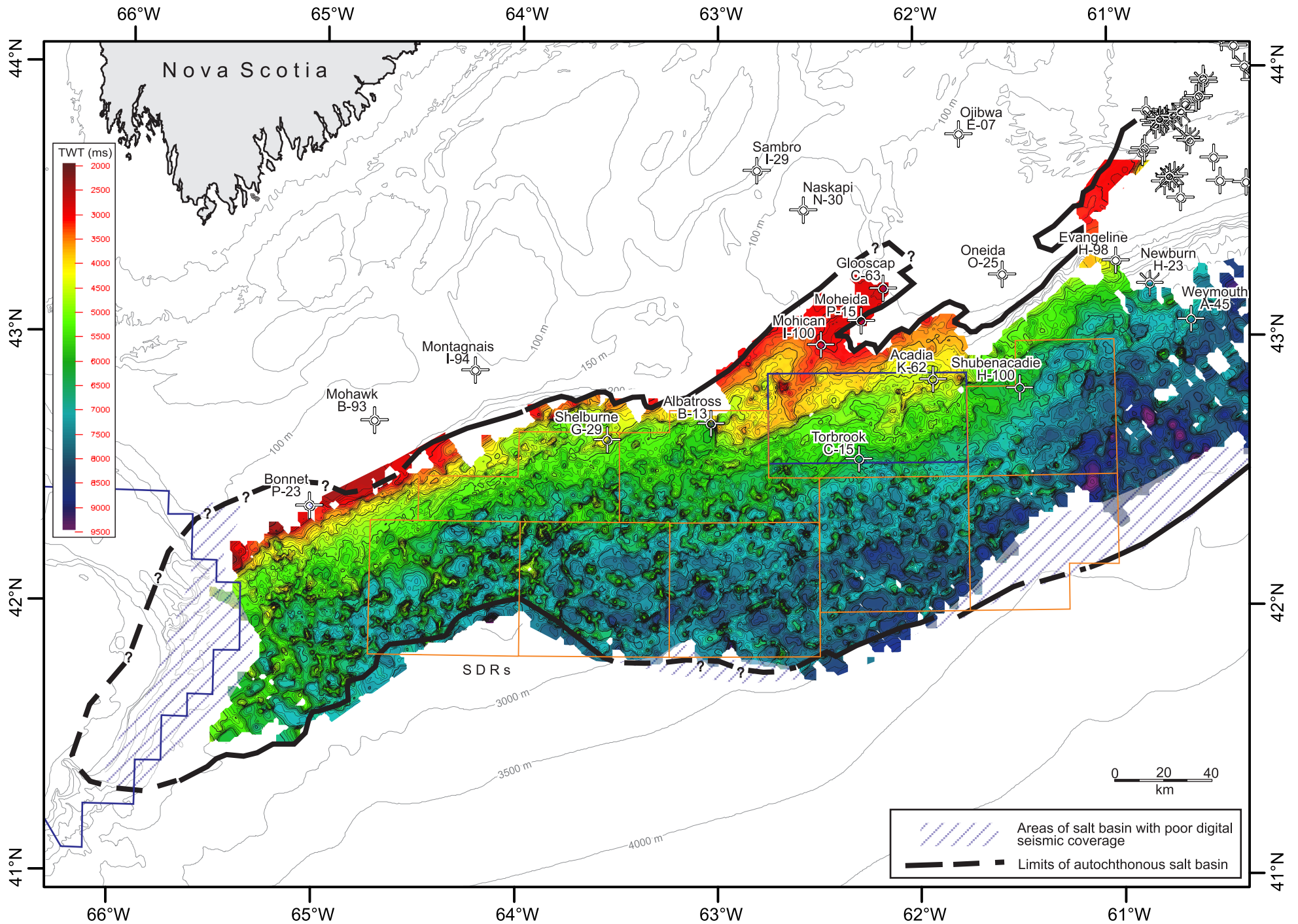
Figure 13a – Gridded time-structure map on the top autochthonous salt surface, correlated along the equivalent primary weld.
