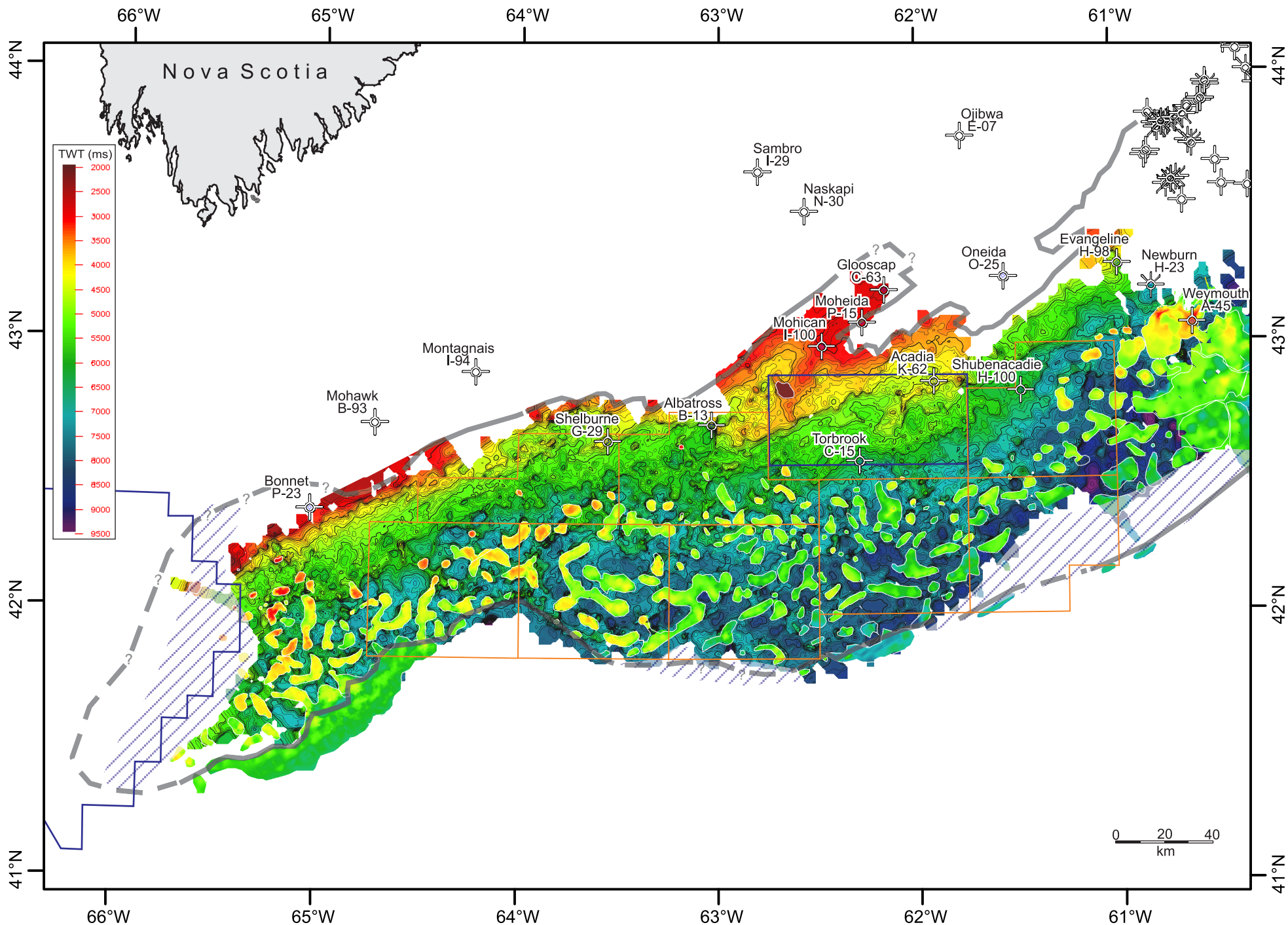
Figure 13b – Gridded time-structure map on the top autochthonous salt surface, overlain by the gridded surface from the top allochthonous salt bodies located predominantly in the ASM province. Autochthonous salt highs produce a polygonal network of minibasins in the ASM province, many of which form the stocks of overlying allochthonous salt bodies.
