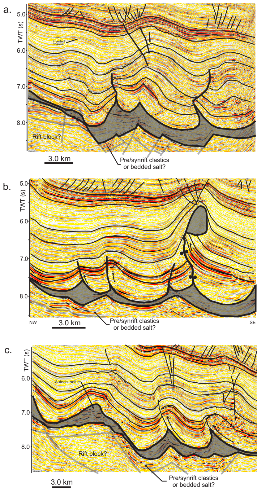
Figure 17 – Three seismic profiles across Jurassic to Cretaceous folds in the landward parts of the ASM province in the eastern study area (see Deptuck, 2008).
