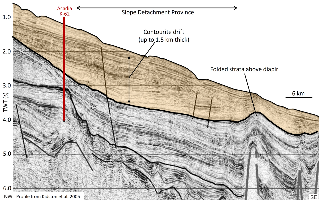
Figure 18 – Northwest- to southeast-oriented profile across a thick contourite drift that is thickest above the SD province. Aggradation of this drift may have prompted down-slope squeezing of pre-existing salt diapirs in the ASM province. Profile from Kidston et al., (2005).
