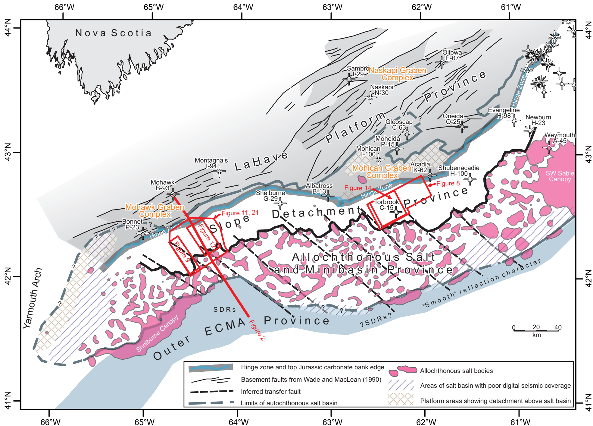
Figure 1a - Map showing key structural elements and four-way post-rift structural subdivision of the western Scotian Margin. Fault traces on the LaHave Platform are from Wade and MacLean (1990). Note that parts of the autochthonous salt basin underlie the LaHave Platform, Slope Detachment, and Allochthonous Salt and Minibasin provinces. Some parts of the autochthonous salt basin have poor data coverage and hence its margins in these locations are poorly constrained. See text for details.
