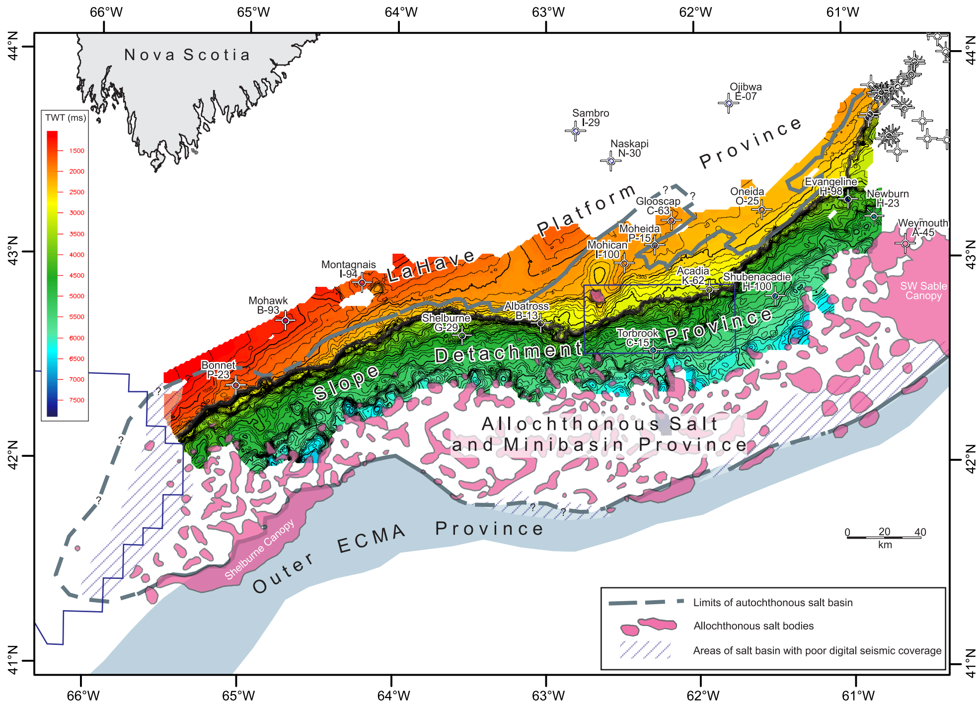
Figure 3 – Gridded time-structure map on the top of the Jurassic carbonate bank.
