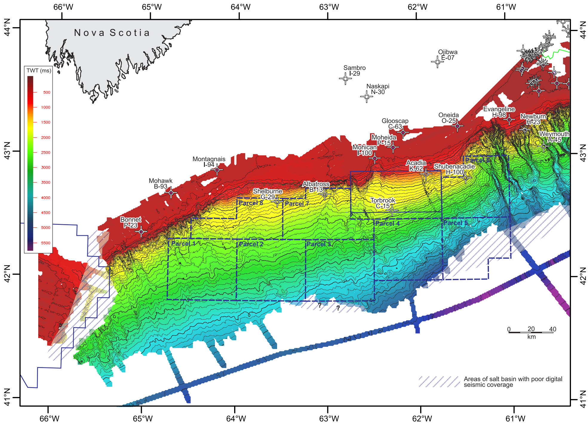
Figure 4a – Gridded time-structure map of the sea floor marker, showing parcel locations.
