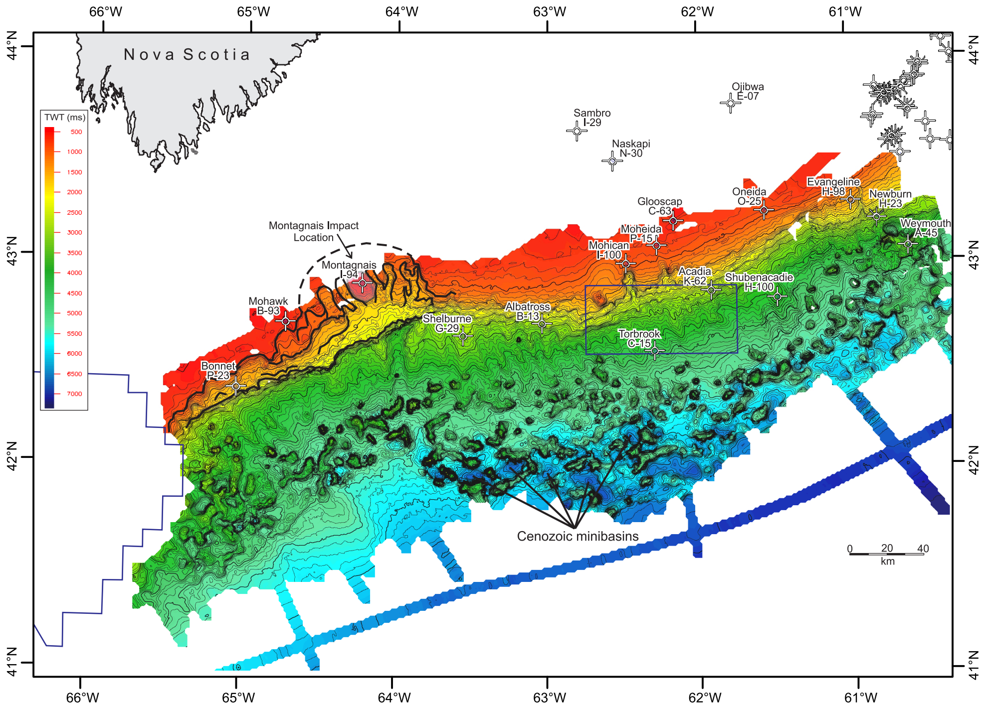
Figure 5a – Gridded time-structure map of a prominent Early Eocene unconformity that formed, at least in part, in response to a 50.8 Ma bolide impact. Scarps and canyon heads within the impact crater are highlighted.
