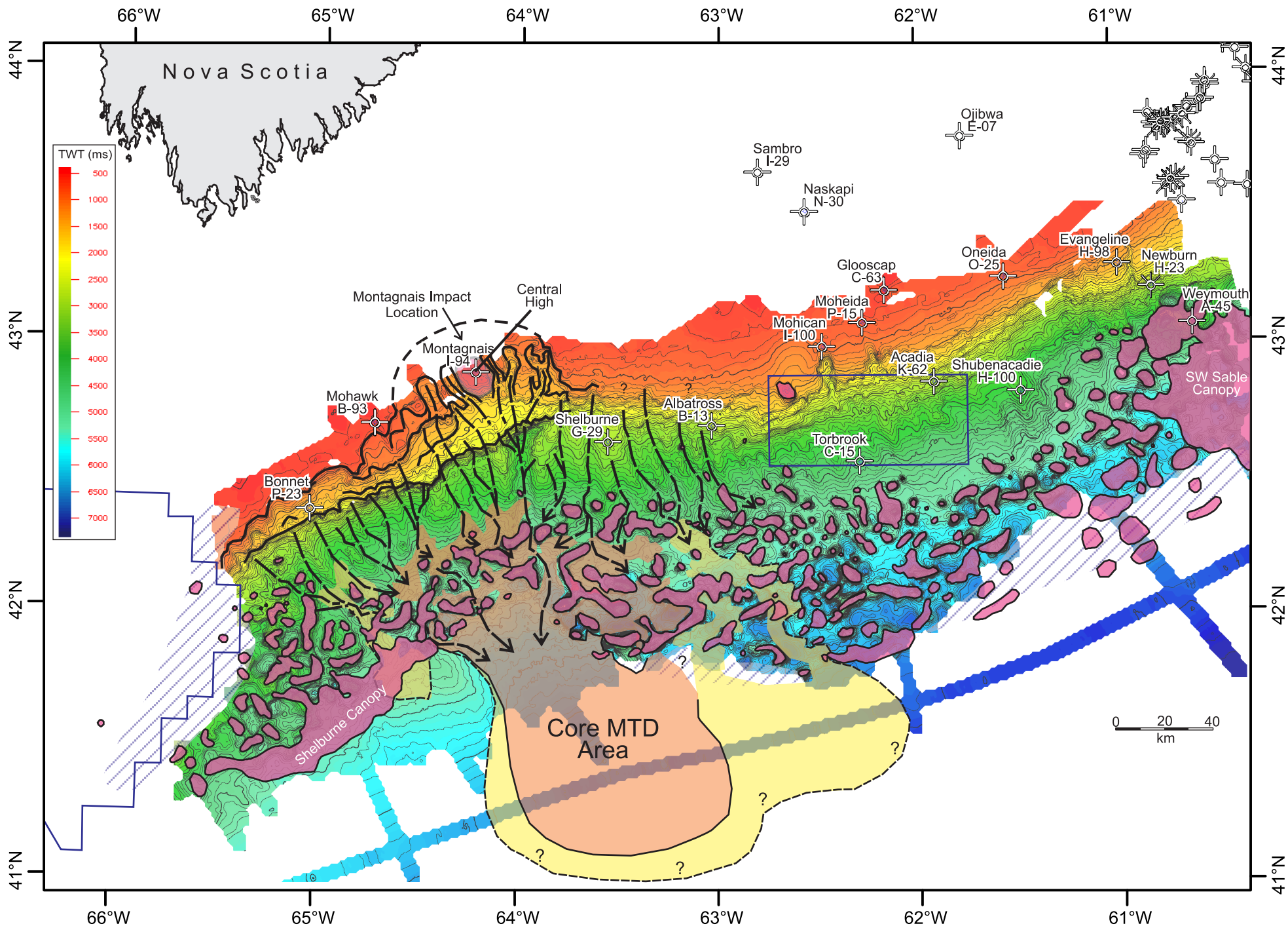
Figure 5b – Gridded time-structure map of the Early Eocene unconformity, annotated to show canyons that transported failed material directly down-slope from the impact site, where a widespread mass transport deposit is recognized. Orange indicates the primary core of the mass transport deposit, while yellow indicates peripheral mass wasted material. There is a high degree of uncertainty about its distribution in deepwater.
