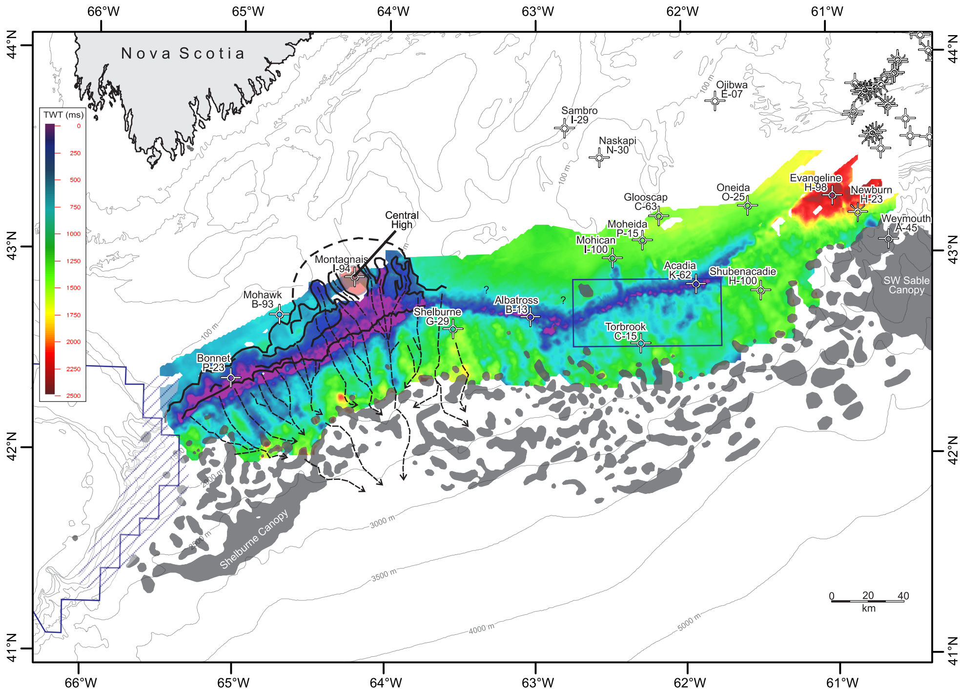
Figure 6 – Time-thickness map between the top Jurassic carbonate bank marker and the Early Eocene unconformity, showing the widespread erosion of the Cretaceous to Paleocene stratigraphic succession caused, at least in part, by the bolide impact.
