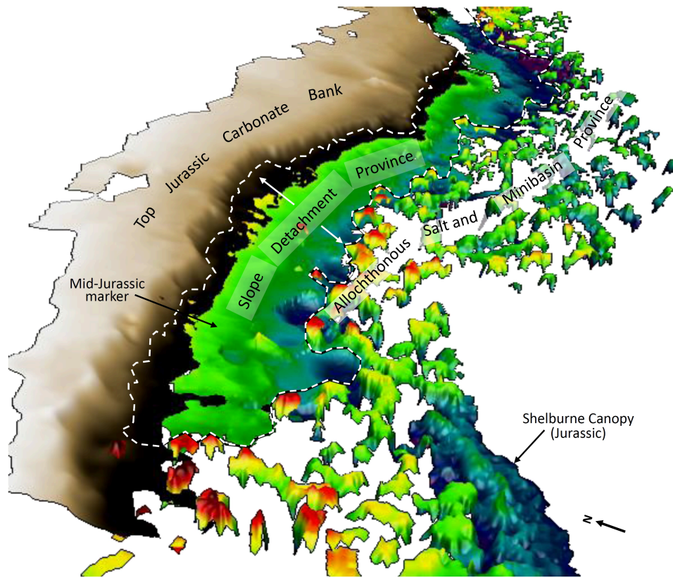
Figure 7 – Perspective view from the southwest showing the relationship between the Jurassic carbonate bank, slope detachment province, and the allochthonous salt and minibasin province. This image illustrates the striking absence of allochthonous salt diapirs in the slope detachment province.
