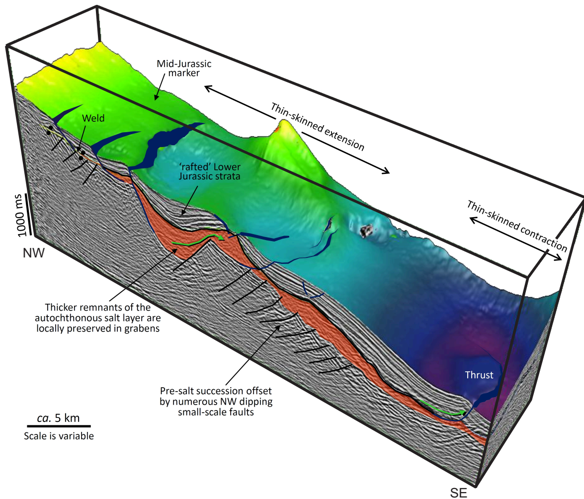
Figure 9 – Perspective view of a mid-Jurassic seismic marker showing thin-skinned detachment and extension above a variably thick autochthonous salt layer, and resulting down-slope contraction that produces a thrust. Basement below the salt is heavily faulted. See Figure 1a for location.
