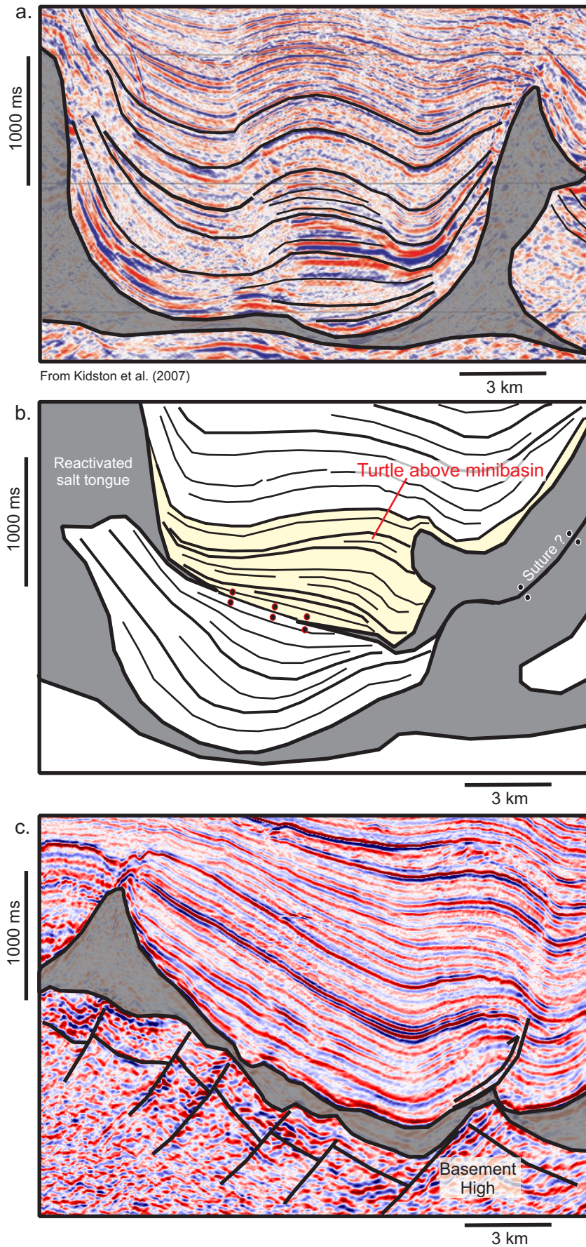
Figure 20 – a) Turtle structure in the ASM province (Parcel 3); b) Unique late turtle structure (yellow) perched above a minibasin (Parcel 4); c) Inverted minibasin near the transition of the SD and ASM provinces (Parcel 1) formed as shortening accommodated up-slope gravity gliding.
